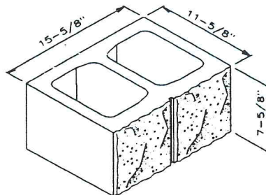
12 x 8 x 16 Scored Split 1-Score
