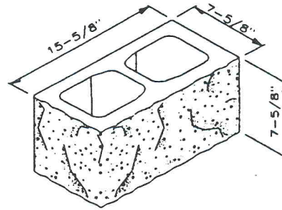
8 x 8 x 16 Splitface Corner
