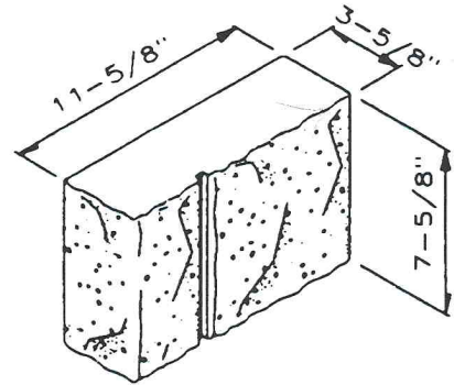
4 x 8 x 12 Solid 12-Long Corner
