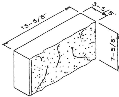
4 x 8 x 16 Splitface
