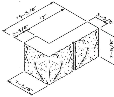
4 x 8 x 16 Solid L Corner
