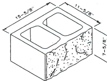
12 x 8 x 16 Splitface
