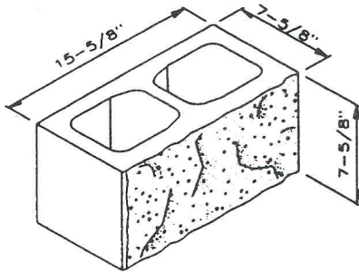
8 x 8 x 16 Splitface
