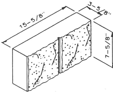
4 x 8 x 16 Scored Split
