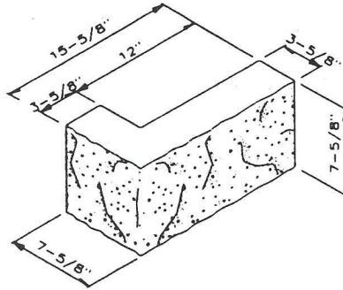
4 x 8 x 16 Splitface Full L Corner
