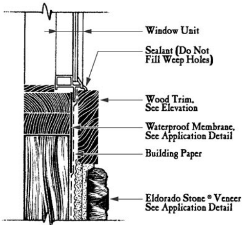
WINDOW SILL Wood Trim
