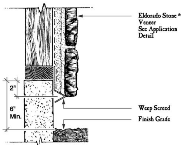
WEEP SCREED
