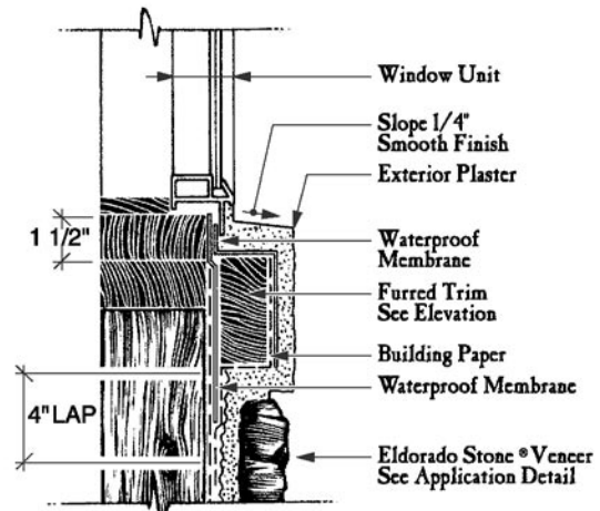
WINDOW SILL Furred Trim
