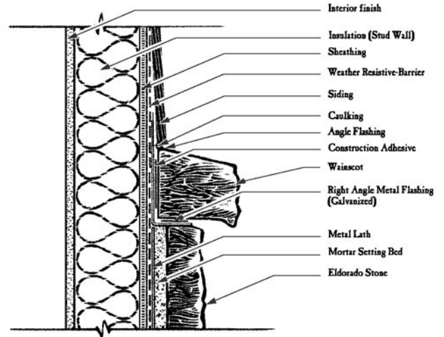
WAINSCOT SILLS
