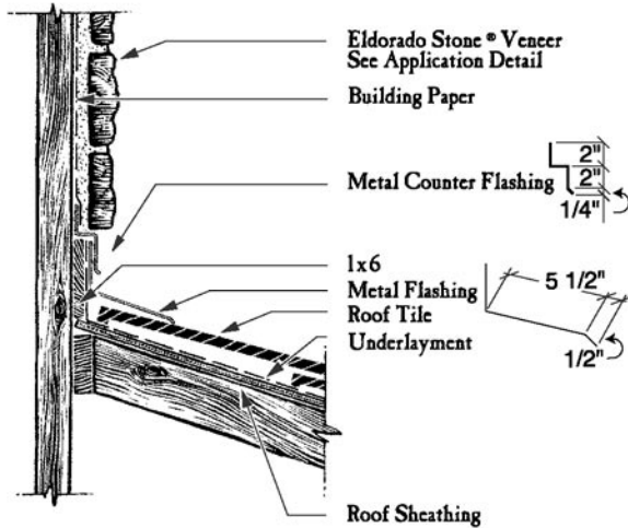
TRANSITION Roof to Wall
