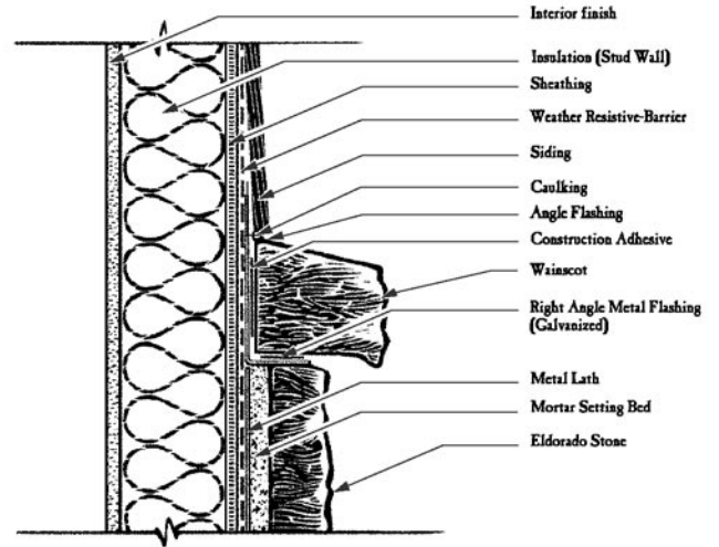
WAINSCOT SILLS
