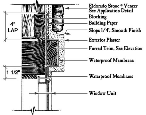
WINDOW HEADER Furred Trim
